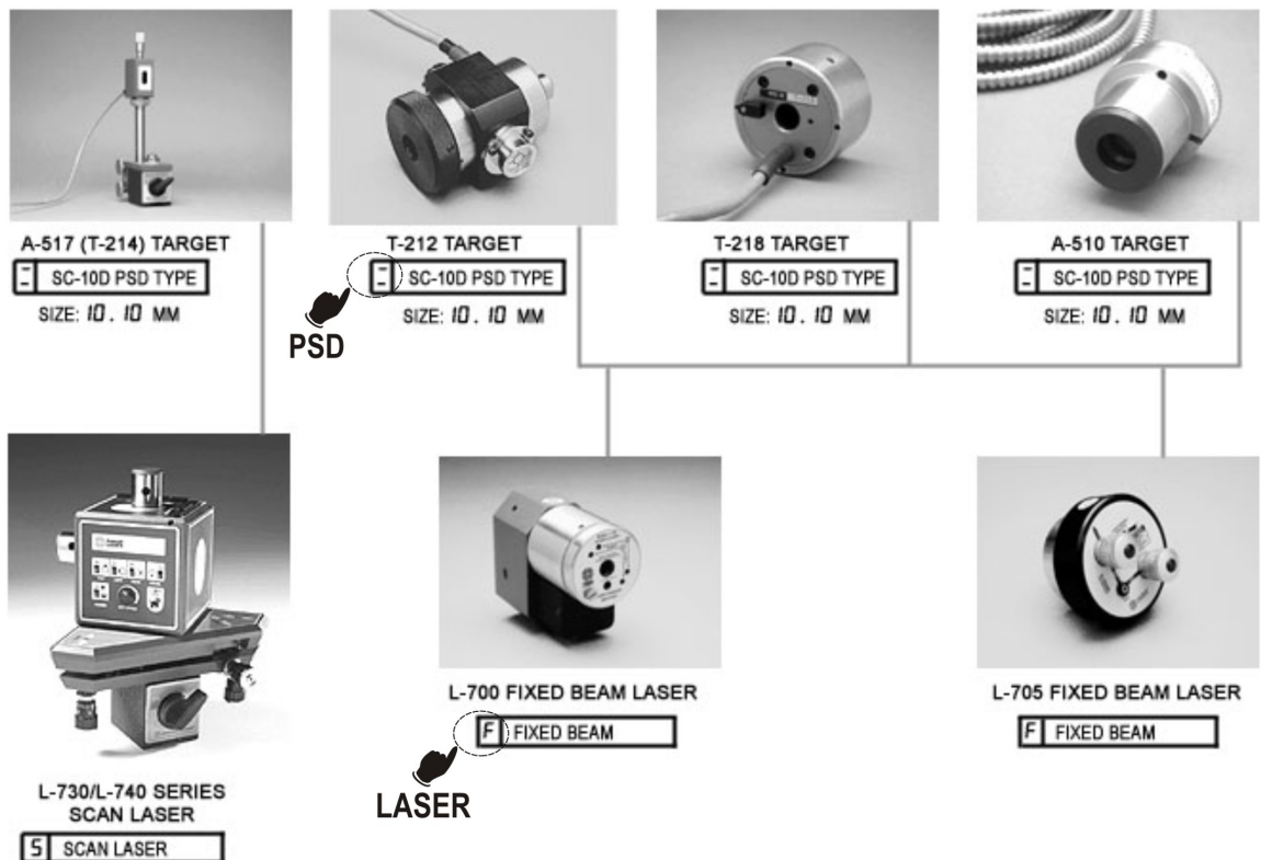
Figure 17 – Target PSD Descriptor, Standard Targets and Lasers
