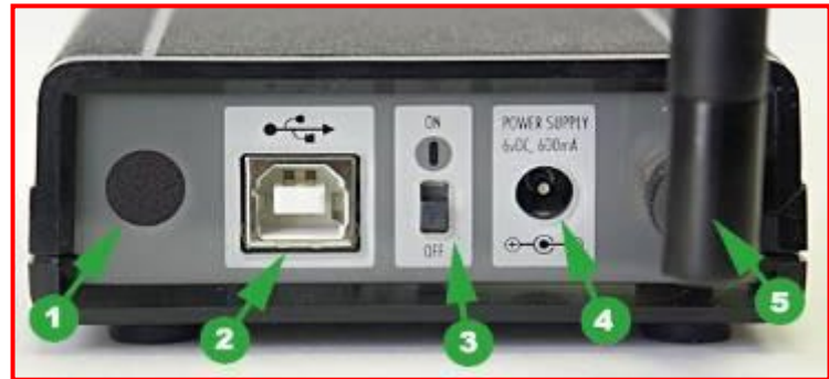
Figure 19 – The A-910 Radio Transceiver/Hub REAR PANEL
